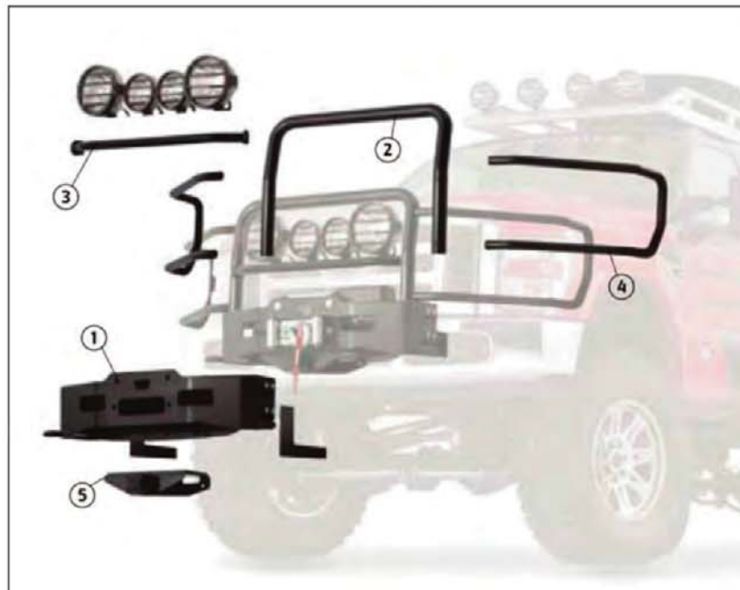
Gen II Trans4mer system, complete with all options.
